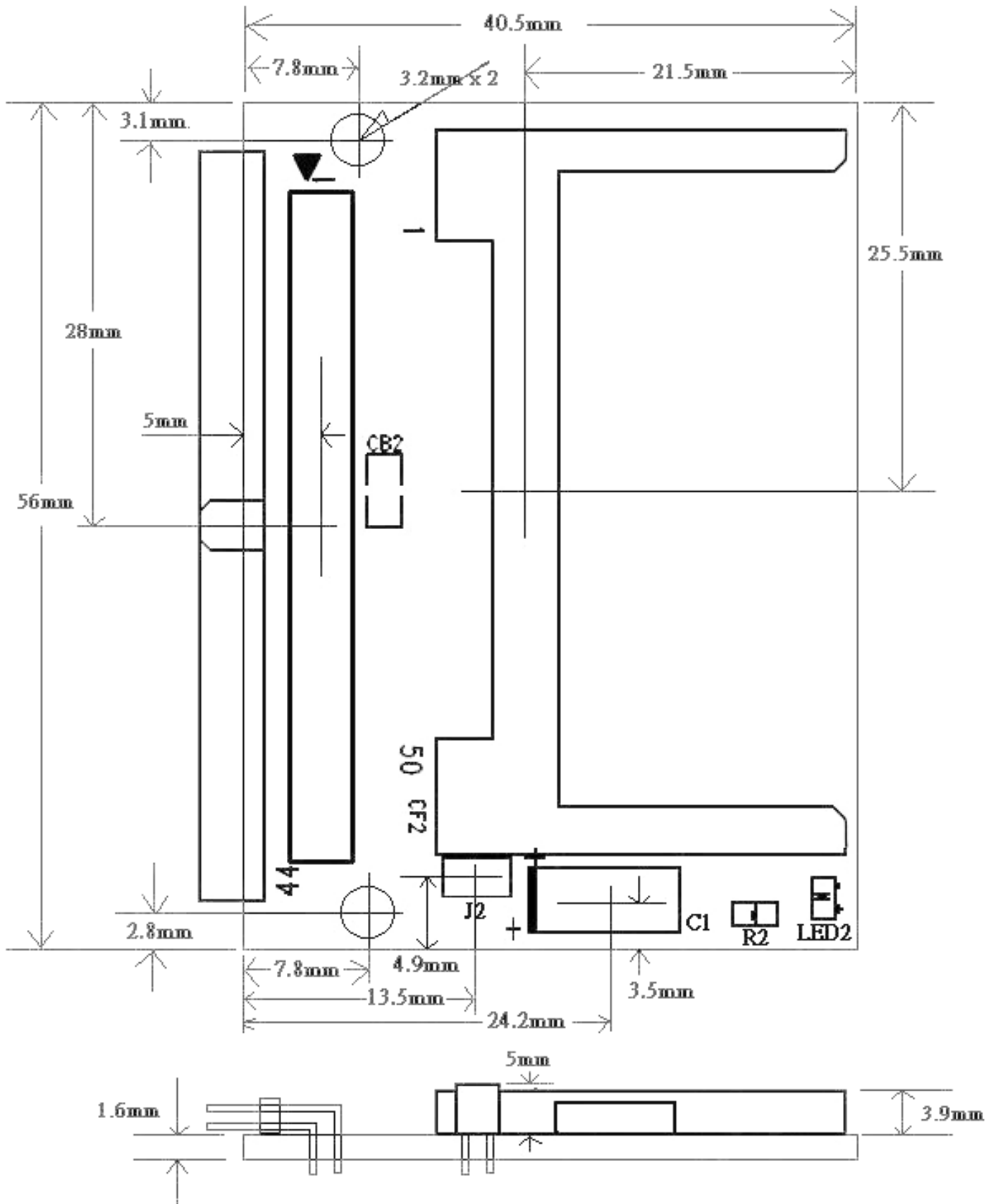
AD44MIDECF mechanical drawing
