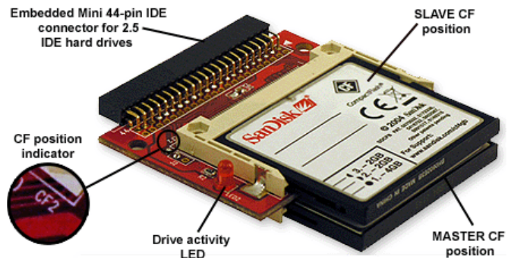
Embedded 44-pin Dual CF-IDE Adapter (model: ADEB44IDE2CF)
