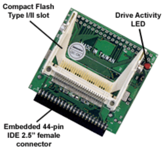
Embedded 44-pin IDE-CF Adapter (model: ADEB44IDE2CF)
